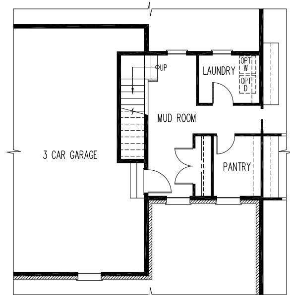
OPTIONAL BONUS ROOM STAIRS
