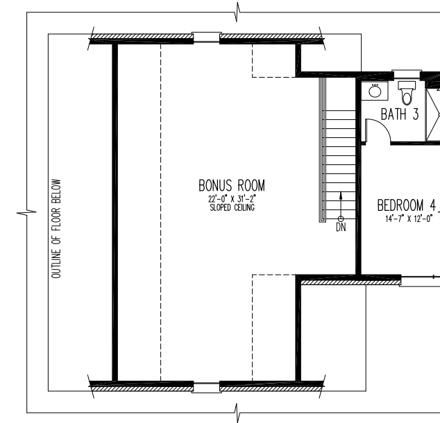
OPTIONAL BONUS ROOM
